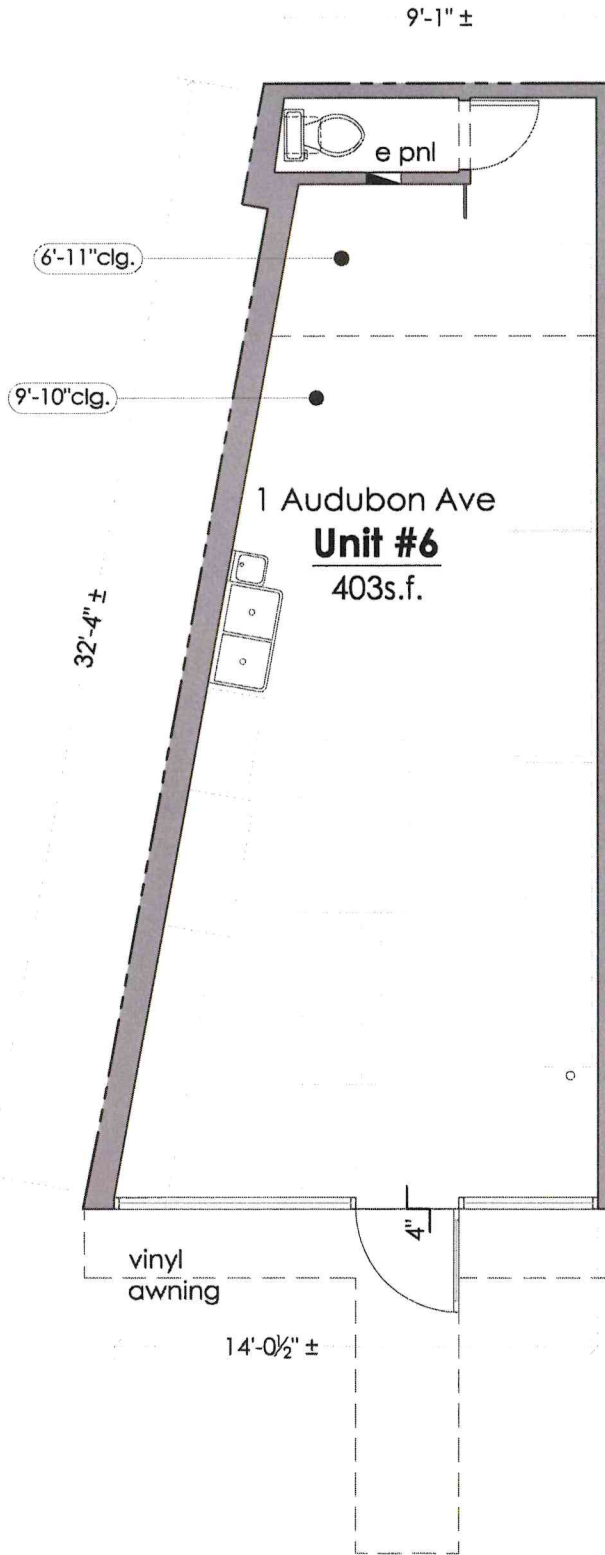
Existing Sketch Layout scale: 3/16"=1'-0"
