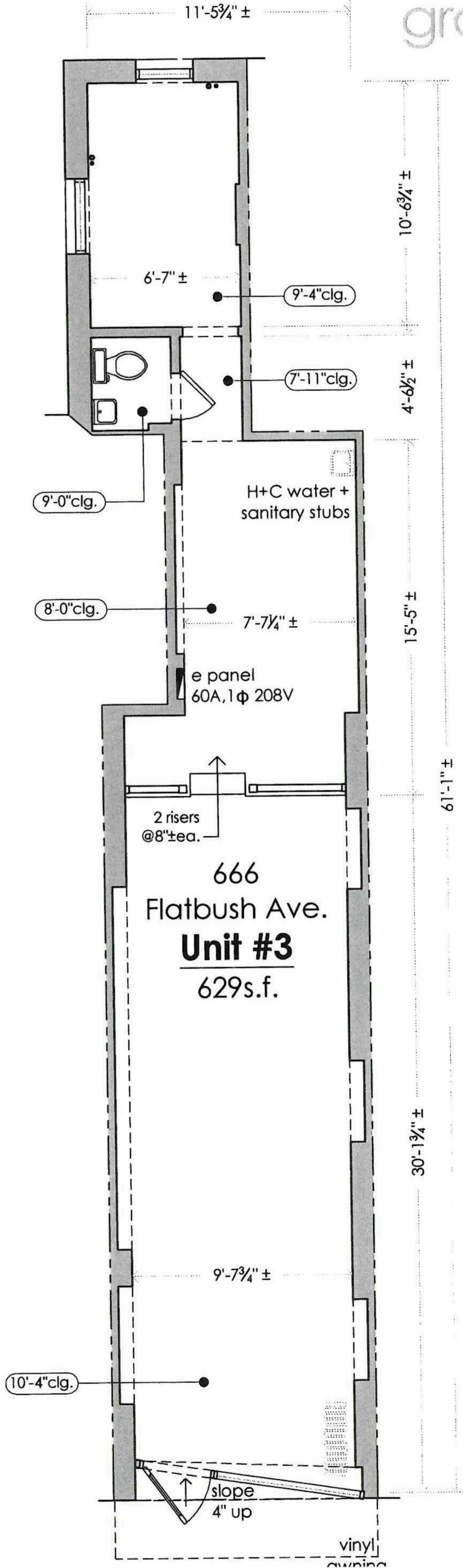
Existing Sketch Layout scale: 3/16"=1'-0"
